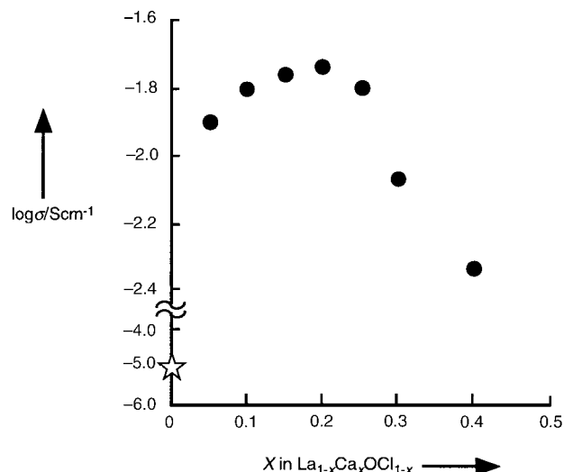
Figure 2. Electrical conductivity at 800°C as a function of x in \text{La}_{1-x}\text{Ca}_x\text{OCl}_{1-x} . The conductivity of pure \text{LaOCl} is also plotted (★).
