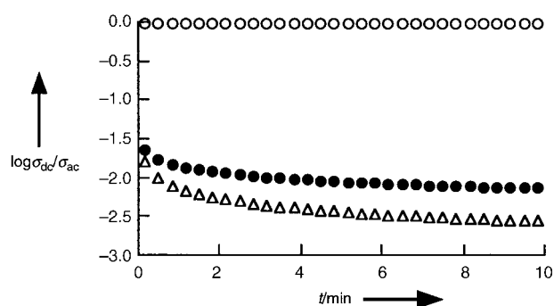
Figure 4. Polarization measurements for the \text{La}_{0.8}\text{Ca}_{0.2}\text{OCl}_{0.8} solid solution in \text{O}_2 (●), \text{He} (△), and 1 vol% \text{Cl}_2 in \text{N}_2 (○) at 700^\circ\text{C} .
